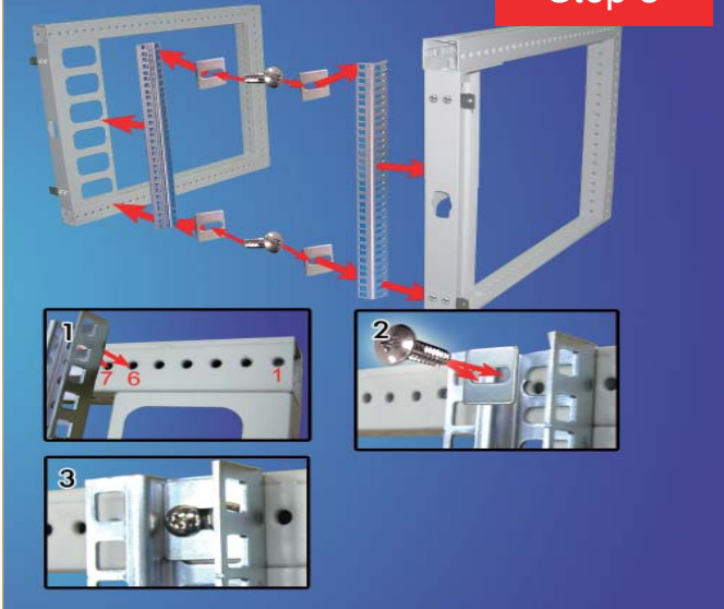
Step 3 Assembly f-shaped mounting angles
