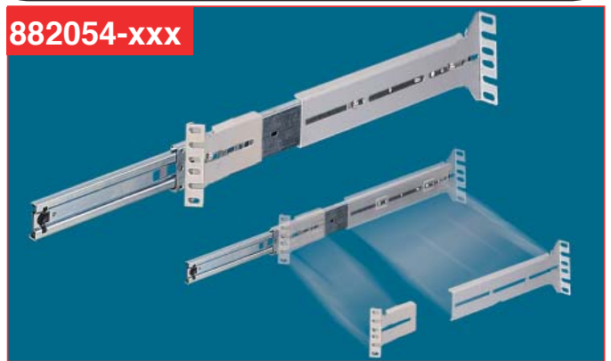
3 Sections Telescopic Server Ball-Bearing Rail for ODD "U" Components
