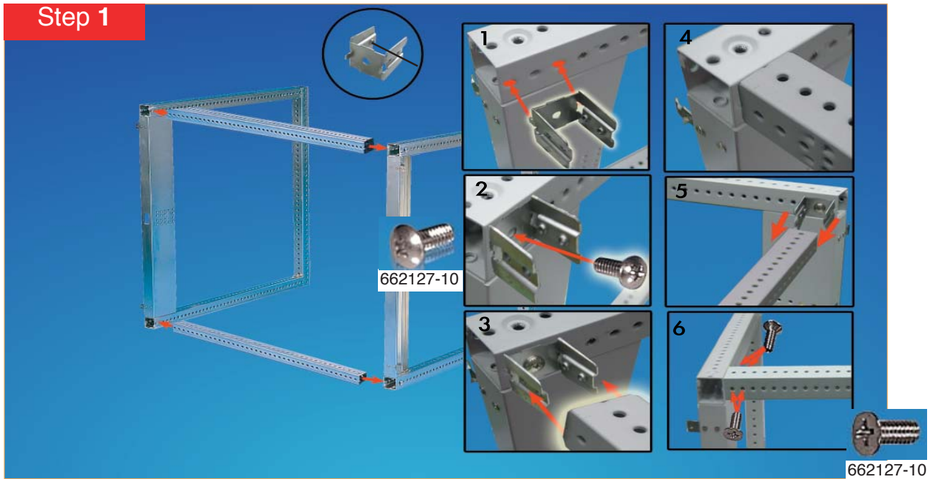
Step 1 Assembly Main Frames :
