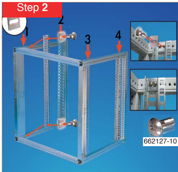
Step 2 Assembly F-shaped Mounting Angles :
