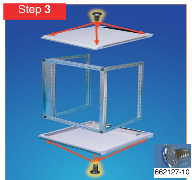
Step 3 Assembly Roof & Bottom Panels
